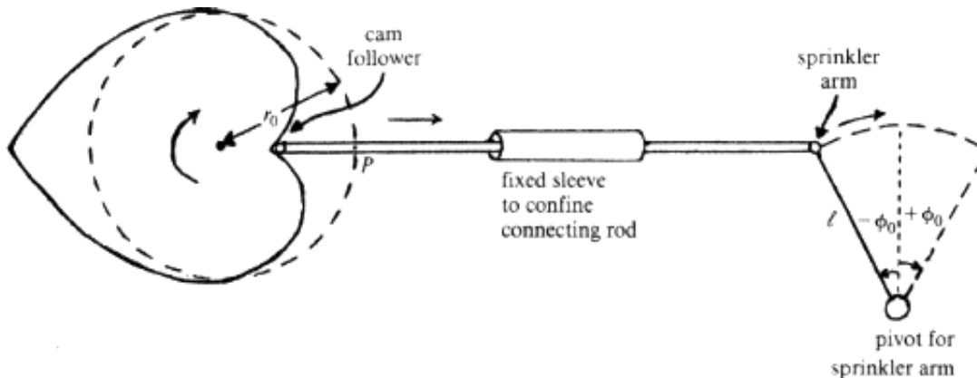
Figure 4. A typical cam mechanism
