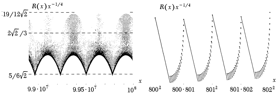
FIGURE 4 Big bounces and small stutters for R(x)x^{-1/4} .
