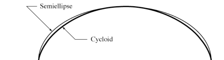
Figure 2. A comparison of the cycloid and semiellipse.
