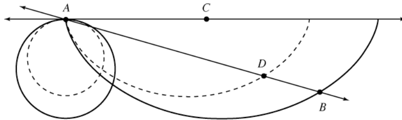
Figure 11. Newton's solution.
